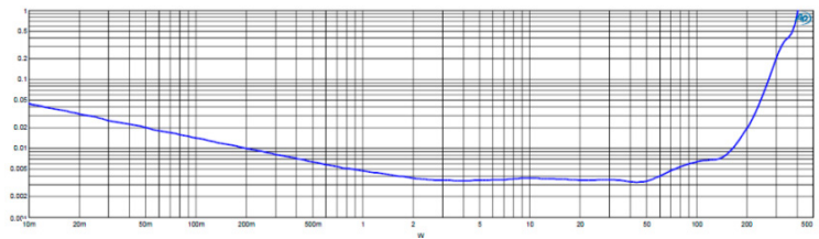
THD vs. Power (1 kHz, 4 Ω)
