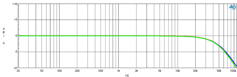
Frequency response (8 Ω, 4 Ω, and open circuit):
