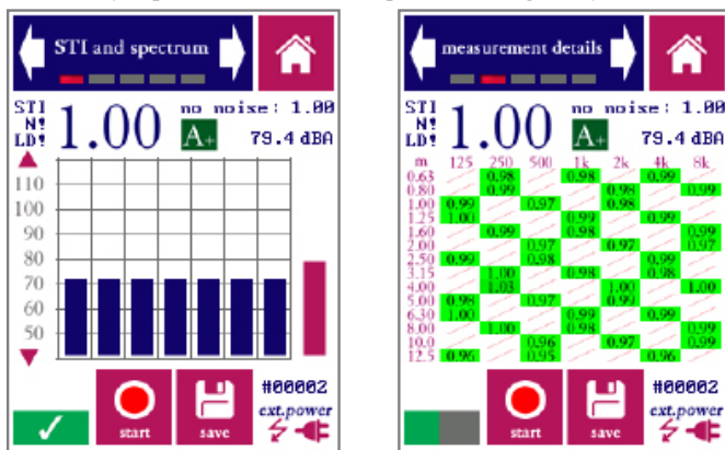
Full STI measurement result (left) and MTF details (right)
