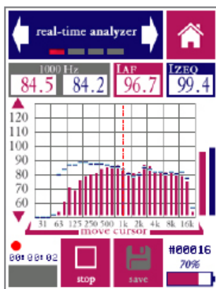
RTA main measurement screen (1/3 octave band mode)
